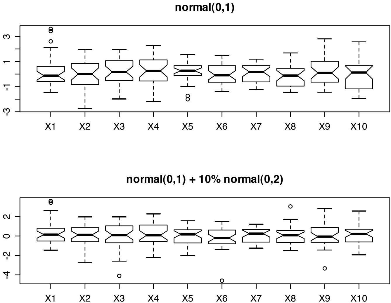
Figure 2. Alternatively, the figure can be made a large figure by using the figure* command. This figure was generated using the R statistics and graphics program. This is a demonstration of a 'notched boxplot' for ten samples taken from a normal distribution, and ten taken from a mixture of two normals with different variances.
