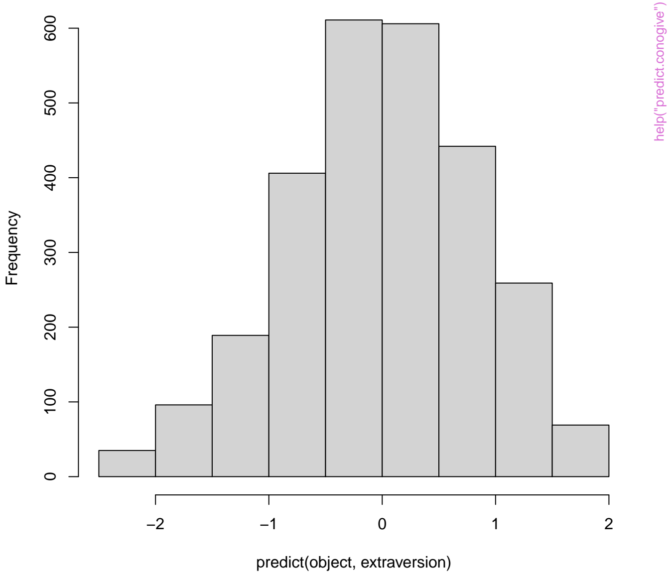
Histogram of predict(object, extraversion)
