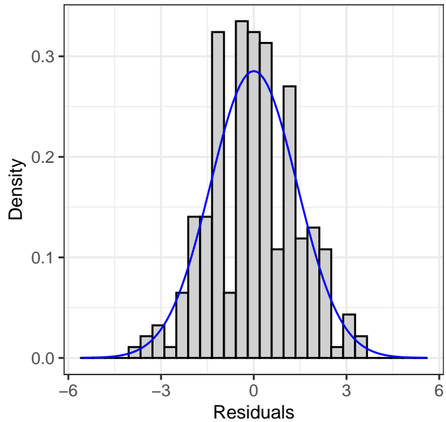
Histogram
