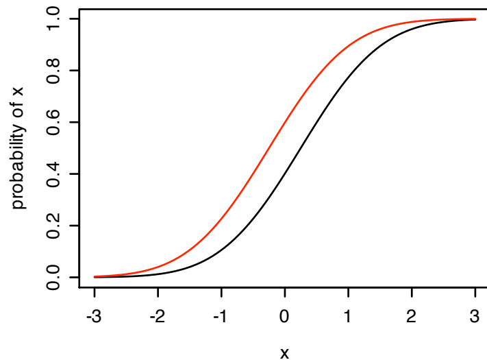
Cumulative normal density for two groups
